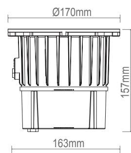
LED body
